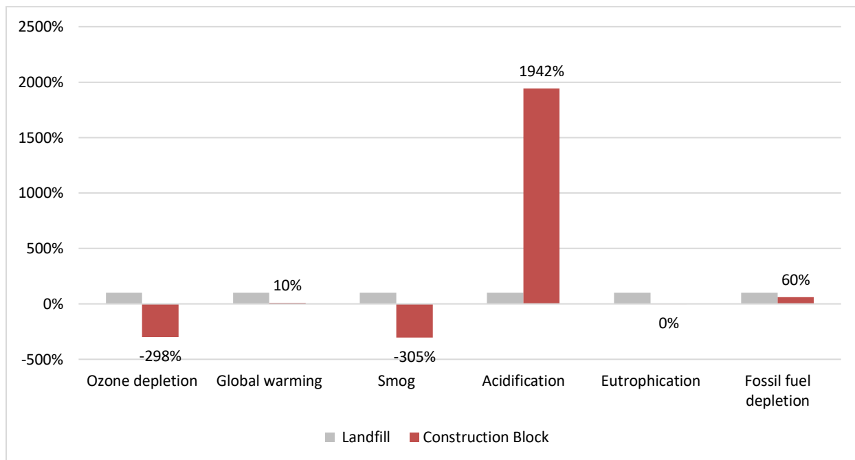
Figure 6.6 – Construction Block and Landfill Relative End-of-Life Impacts
