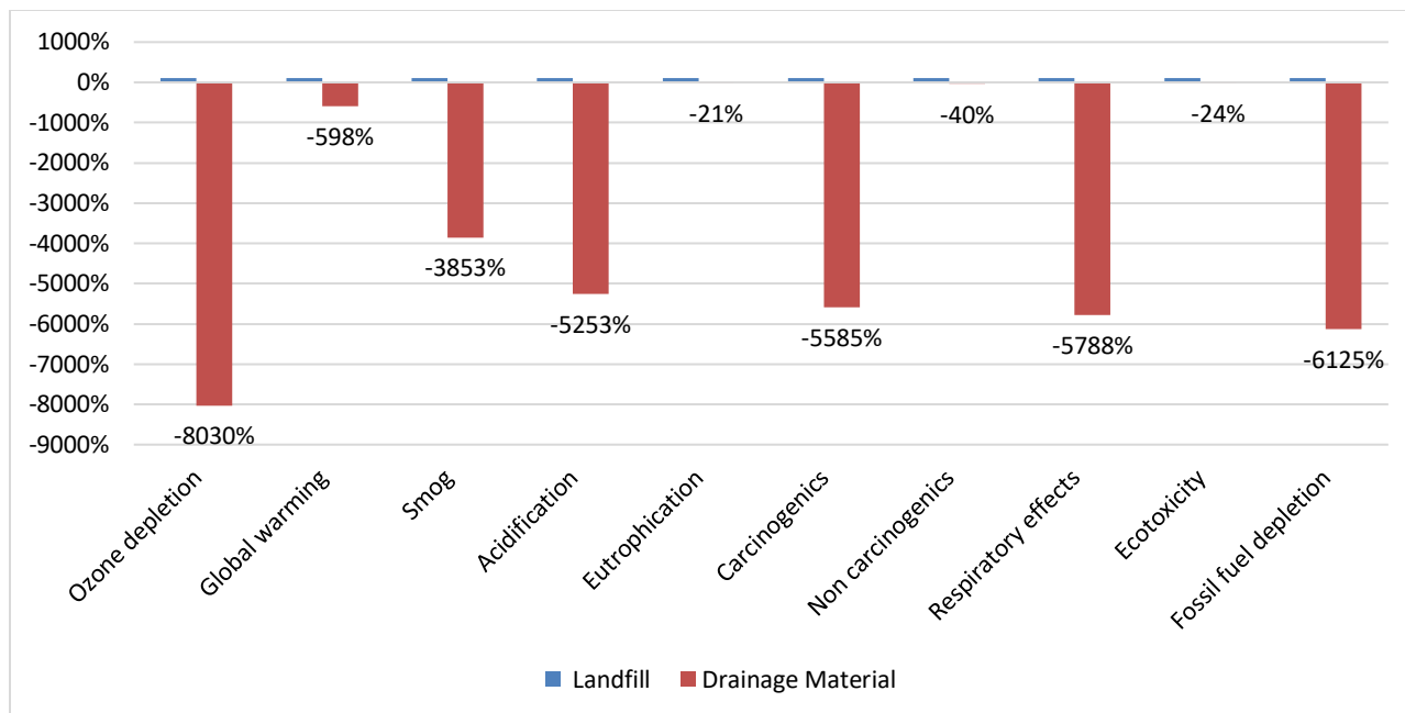
Figure 6.10 – Drainage Material and Landfill Relative End-of-Life Impacts
