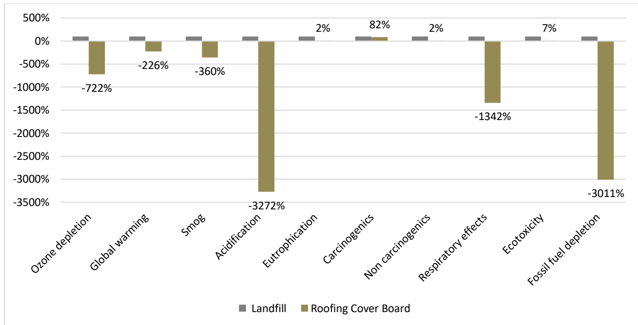
Figure 6.8 – Roofing Cover Board and Landfill Relative End-of-Life Impacts
